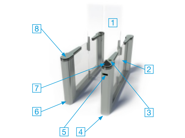
1. Flap Leaves. 2. Glass inlay. 3. Pictogram. 4. Plinth. 5. LED way mode indicator. 6. End Leg. 7. Card reader integration. 8. Lid.
